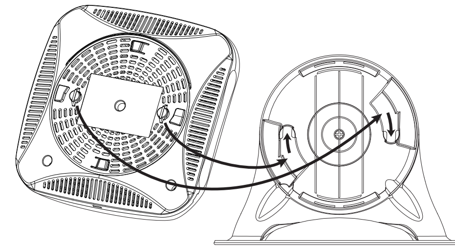
Figure 3 Stand Installation
